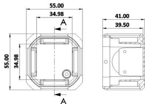
OUT DOOR WALL LIGHT SMALL 4 WAY
