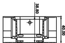
WALL LIGHT 3 WAY ROUND
