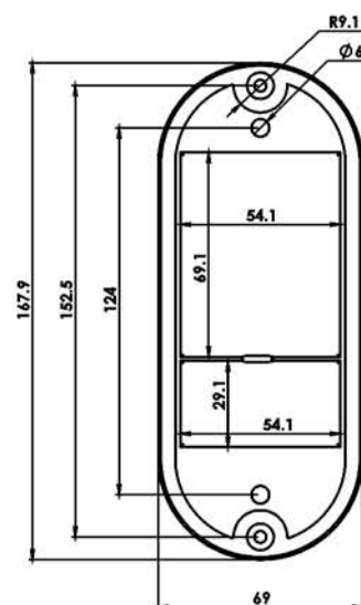
ECONOMY BULK HEAD - SMALL
