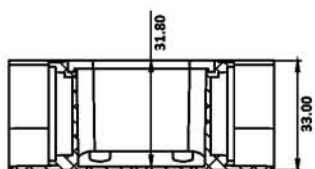
WALL LIGHT 1 WAY ROUND
