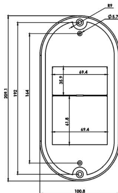
ECONOMY BULK HEAD - BIG
